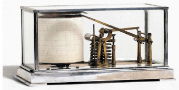
Seven-Capsule Gilt Brass Barograph, Holosteric Model with Chrome Case
