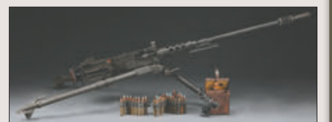
Well Accessorized And Highly Collectible WWII Savage Arms Corporation U.S. M2 Heavy Barreled .50 Bmg Machine Gun (Curio & Relic).
