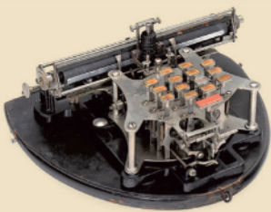
»Viktoria (Gardner)«, 1890 German Version of the English type sleeve machine by John Gardner, Manchester, UK. – Extremely rare collector's item. Estimate: € 10,000 – 15,000 / US$ 11,000 – 16,500
